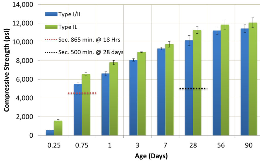
Figure 4.8. Compressive strength of class AAA concrete from plant A. The GDOT specified strengths for class AAA concrete are shown as dotted lines for 0.75 and 28 days.
