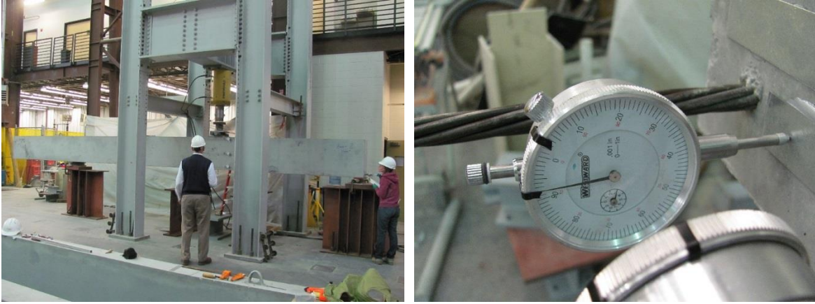
Figure 3.28. Development length test and gages used for measuring strand slip.
