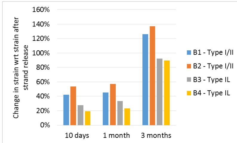
Figure 4.20. Prestress losses with respect to strain values after release.
