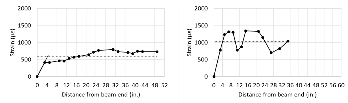
Figure 4.22. Beam 1 (Type I/II) concrete surface strain measurements for transfer length
