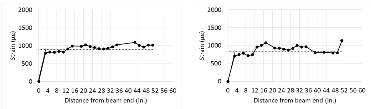
Figure 4.23. Beam 2 (Type I/II) concrete surface strain measurements for transfer length
