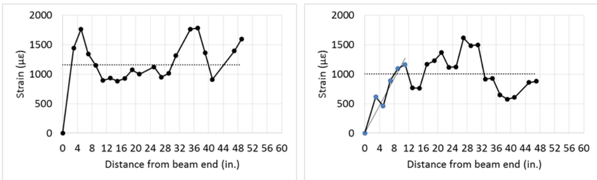
Figure 4.25. Beam 4 (Type IL) concrete surface strain measurements for transfer length
