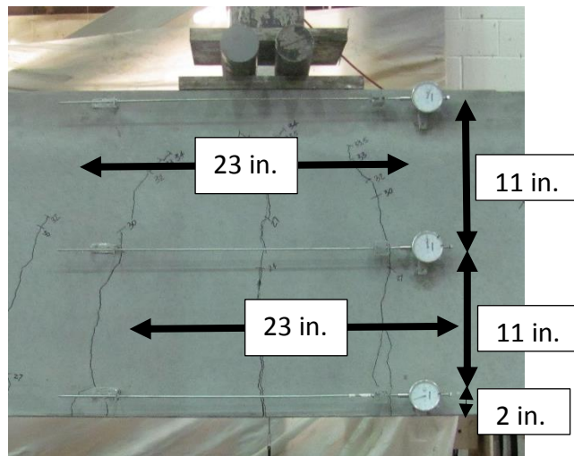
Figure 3.29. Dial gages placement for strain profile measurements under applied load
