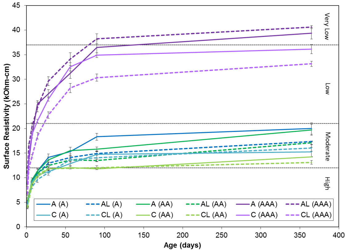
Figure 4.16. Surface resistivity for class AAA concretes made with A, AL, C and CL cements.
