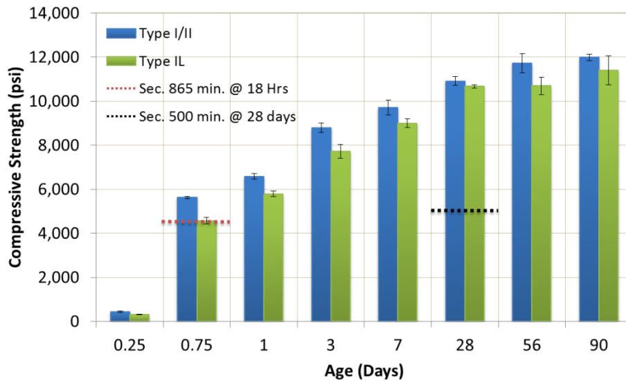
Figure 4.9. Compressive strength of class AAA concrete from plant C. The GDOT specified strengths for class AAA concrete are shown as dotted lines for 0.75 and 28 days.
