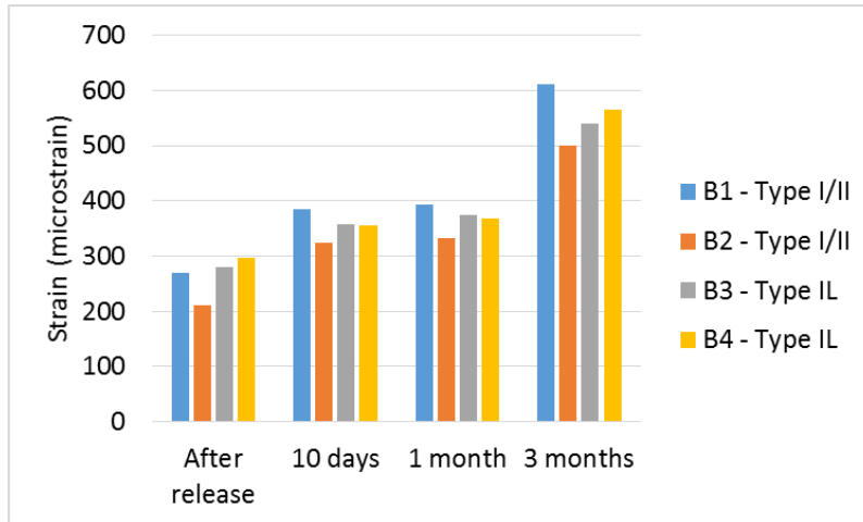
Figure 4.18. Strain values of prestressed beams at level of strands with respect to values taken before release.
