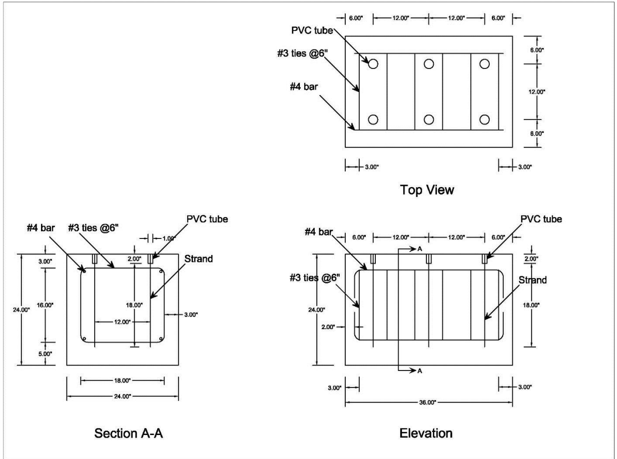
Figure 3.21. Design of concrete blocks for Mustafa test.
