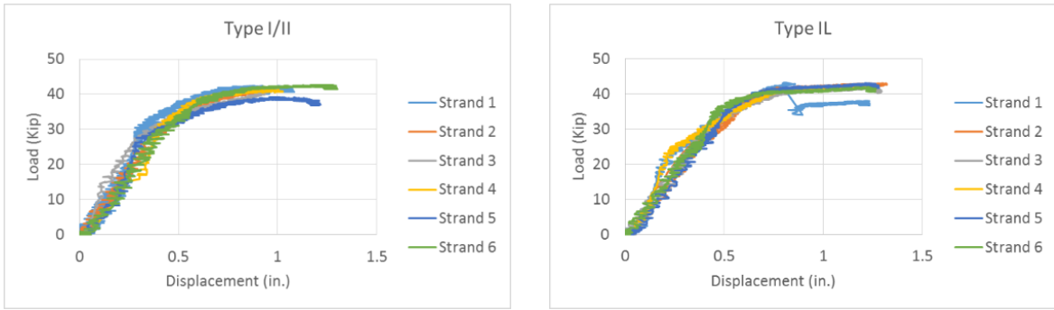
Figure 4.21. Mustafa pull-out test results.
