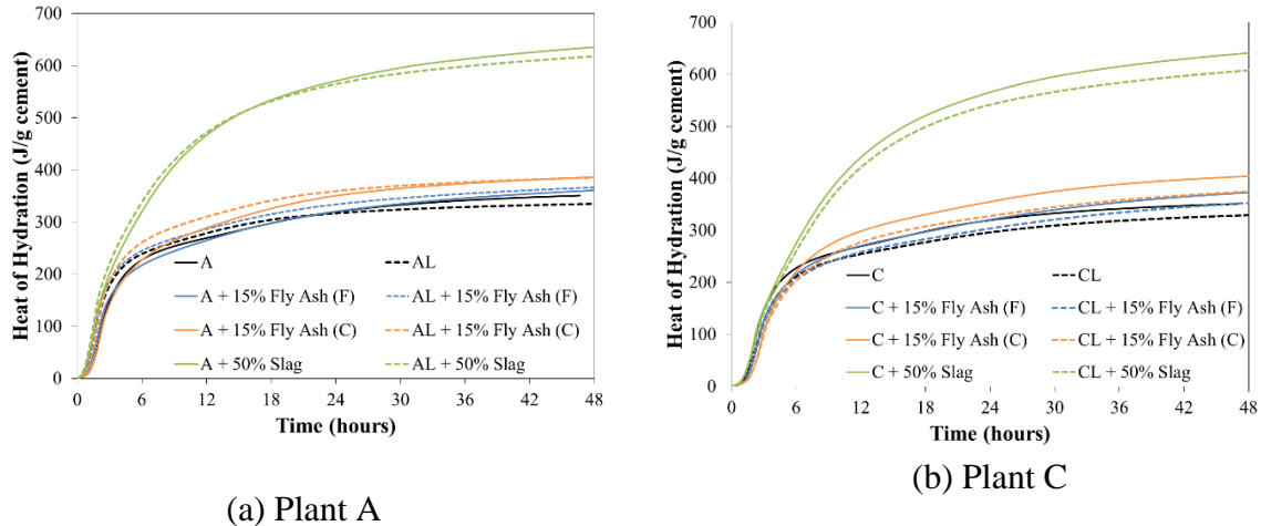
Figure 4.5. Cumulative heat of hydration (power) curves for cements from plants A and C with supplementary cementitious materials (SCMs).
