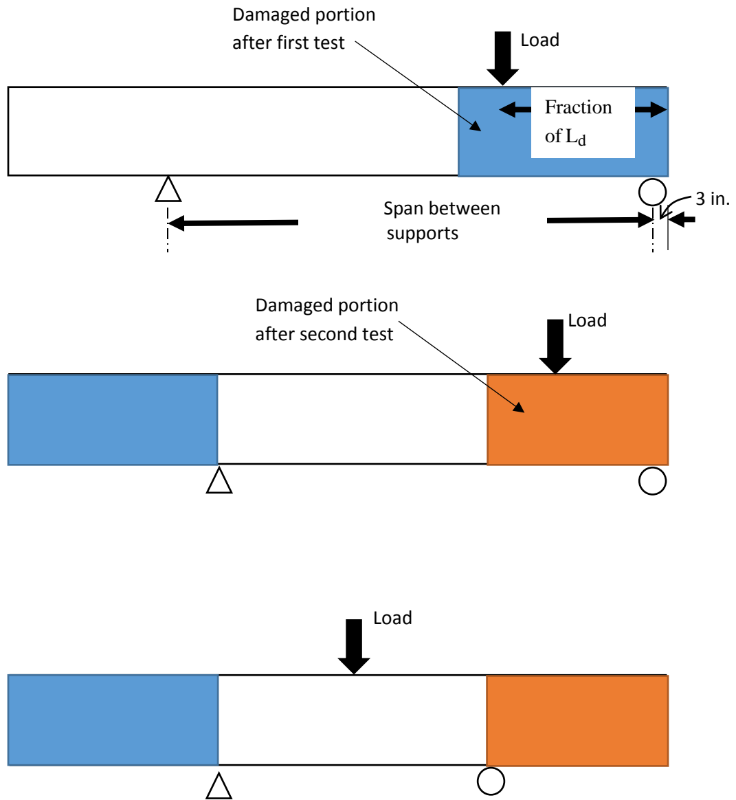
Figure 3.27. Sequence of beam tests
