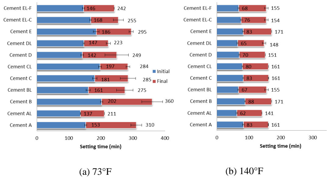
Figure 4.6. Time of setting of cements “A” to “E” at 73°F and 140°F.
