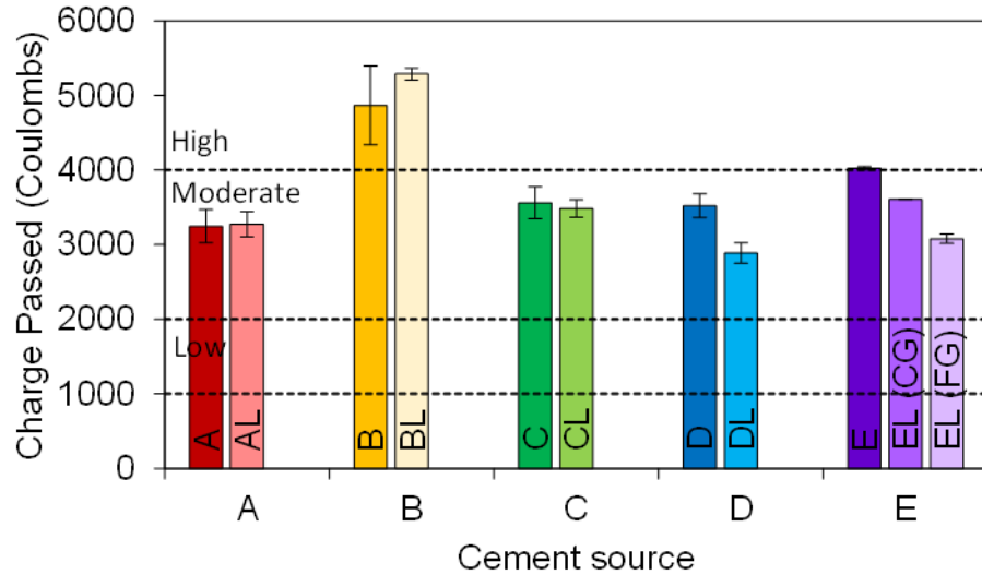
Figure 2.5. Total charge passed by RCPT for concretes A-E, after 56 days of hydration. Error bars indicate the range of values obtained for each mixture.
