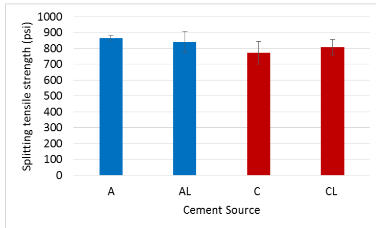
Figure 4.12. Splitting tensile strength of Type I/II and Type IL cements from plants A and C (class AAA concrete)
