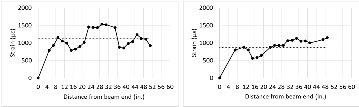
Figure 4.24. Beam 3 (Type IL) concrete surface strain measurements for transfer length
