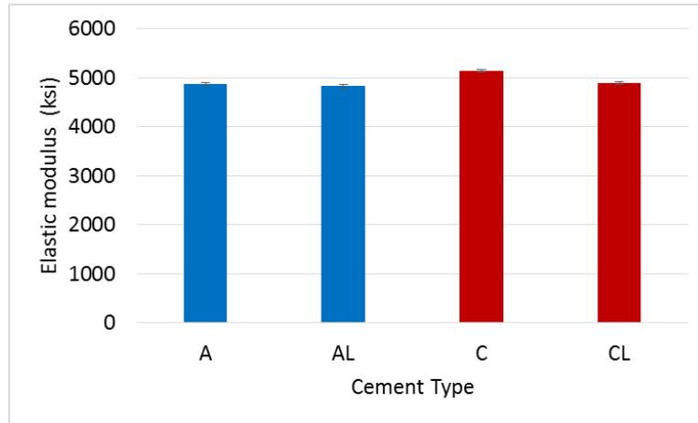
Figure 4.11. Elastic modulus values of Type I/II and Type IL cements from plants A and C (class AAA concrete)
