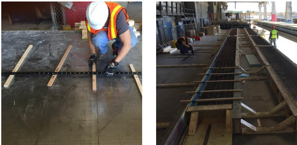
Figure 3.26. Placement of embedded nuts located in steel spacer bar for transfer length measurements.
