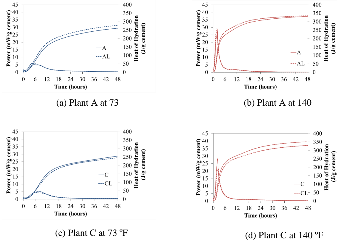
Figure 4.3. Isothermal Calorimetry of cements from plants A and C at 73°F and 140°F.
