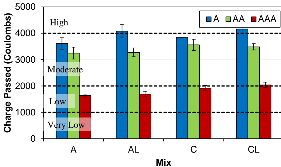
Figure 4.17. Chloride ion permeability (RCPT) for class A, AA, and AAA concretes at 56 days.
