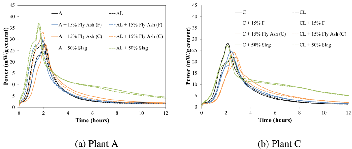
Figure 4.4. Isothermal calorimetry heat evolution curves for cements from plants A and C with supplementary cementitious materials (SCMs).
