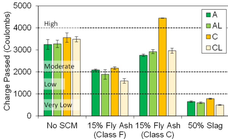
Figure 2.6. Total charge passed by RCPT for concretes containing SCMs, after 56 days of hydration. Error bars indicate the range of values obtained for each mixture.
