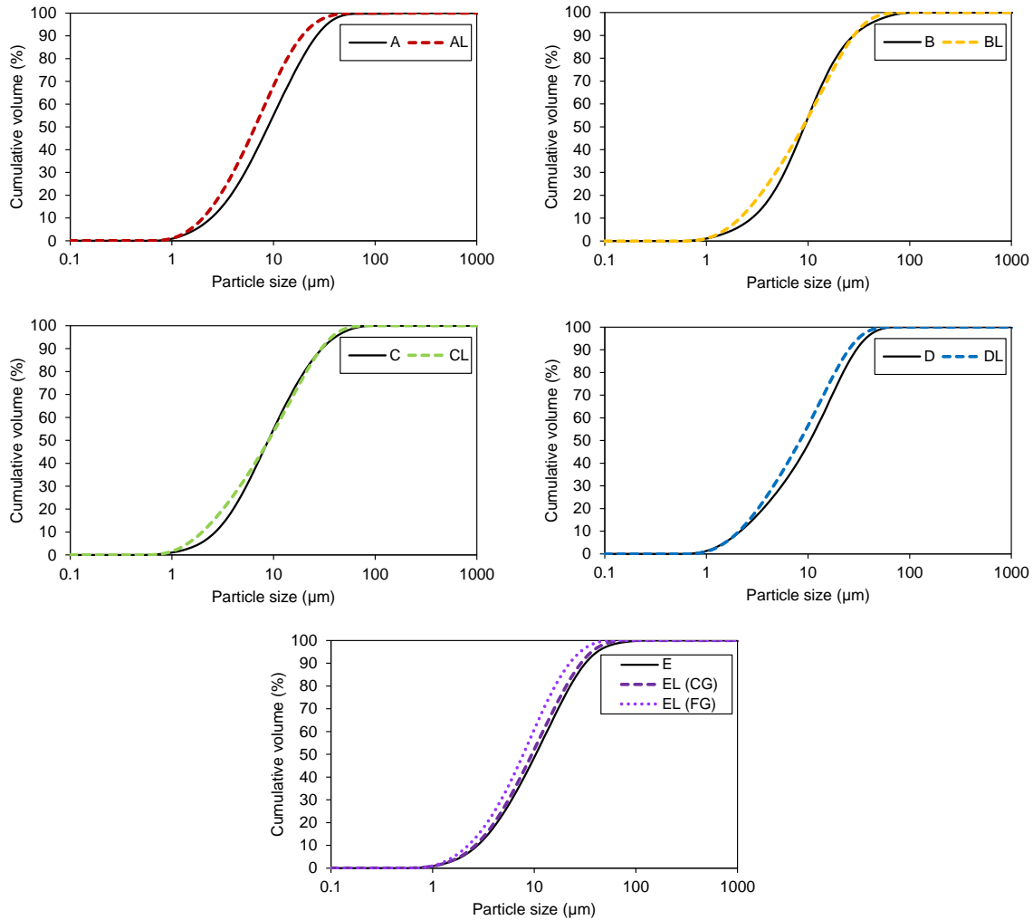
Figure 4.1. Cumulative particle size distribution for cements A to E.
