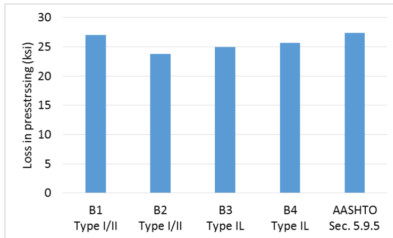
Figure 4.19. Total prestress losses in comparison to AASHTO LRFD [2016] calculations.
