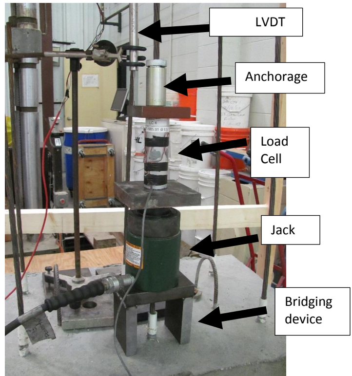
Figure 3.24. Specimen and instrumentation for the Mustafa test.
