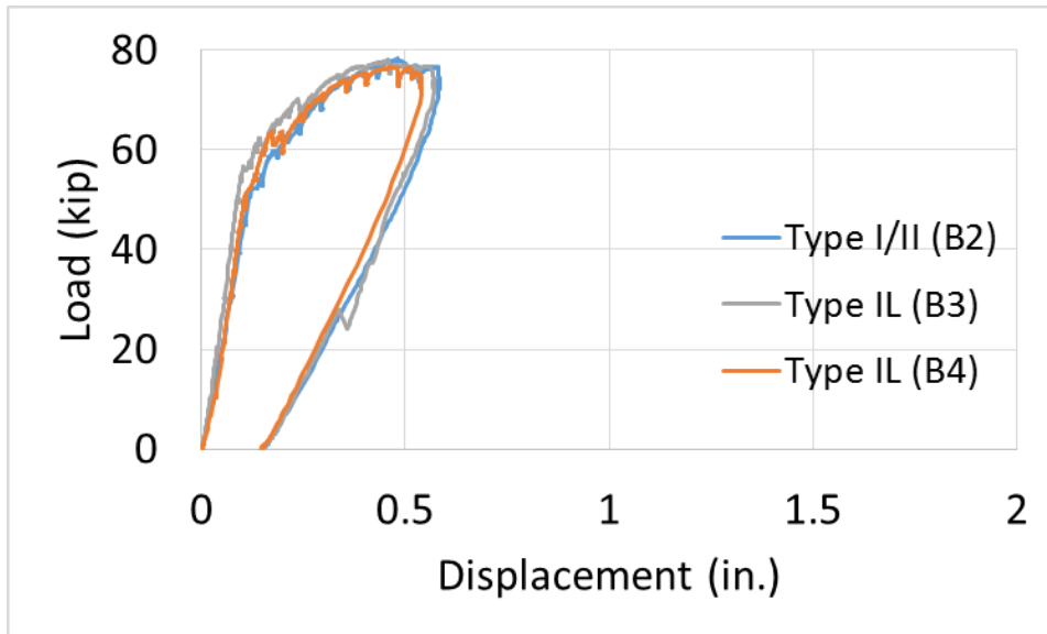
Figure 4.28. Load-displacement results of the flexure test of Beams 2 through 4.
