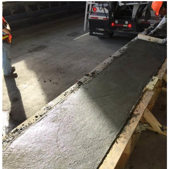
Figure 3.15. Placing concrete and finishing the surface for the beams
