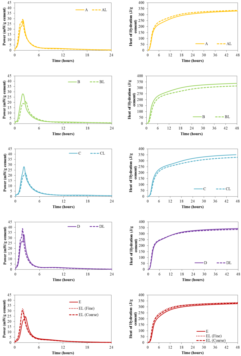
Figure 4.2. Calorimetry results (power and cumulative heat of hydration) for cements A to E at 140°F.
